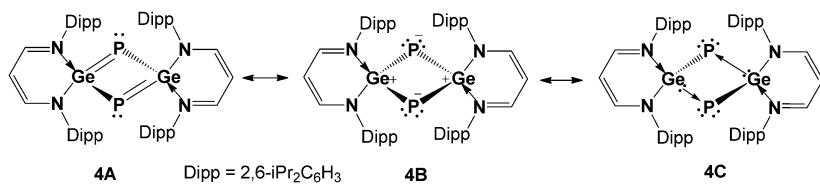
Scheme 3. Resonance structures of 4 .
